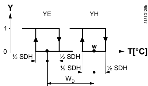
Heating and cooling mode (P01=4)
