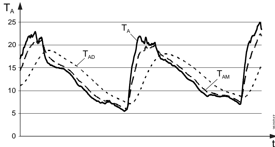
Development of the actual, composite and attenuated outside temperature
